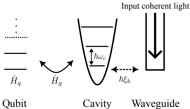
FIG. 1. Schematic picture of system we consider in this study. The system is composed of a qubit, a linear cavity, and a semi-infinite waveguide. In this system, the dynamics induced by a coherent input light is considered.
