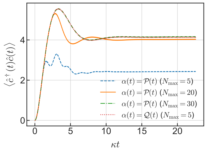
FIG. 7. Time evolution of the cavity photon number of the cavity under a monochromatic drive Ee^{-i\omega_d t} in the transmon case. Initially, |\psi_{\text{ini}}\rangle_{qc} is set to |\tilde{g}, \tilde{0}\rangle . The parameters used in the simulation are (E_C/\hbar\omega_c, E_J/\hbar\omega_c, g/\omega_c, \kappa/\omega_c, N_g, \omega_d/\omega_c) = (5.0 \times 10^{-2}, 1.6, 3.0 \times 10^{-2}, 1.619 \times 10^{-3}, 0.0, 1.0015) . The amplitude of input field E is set to 3.0 \times 10^{-3}\omega_c .
