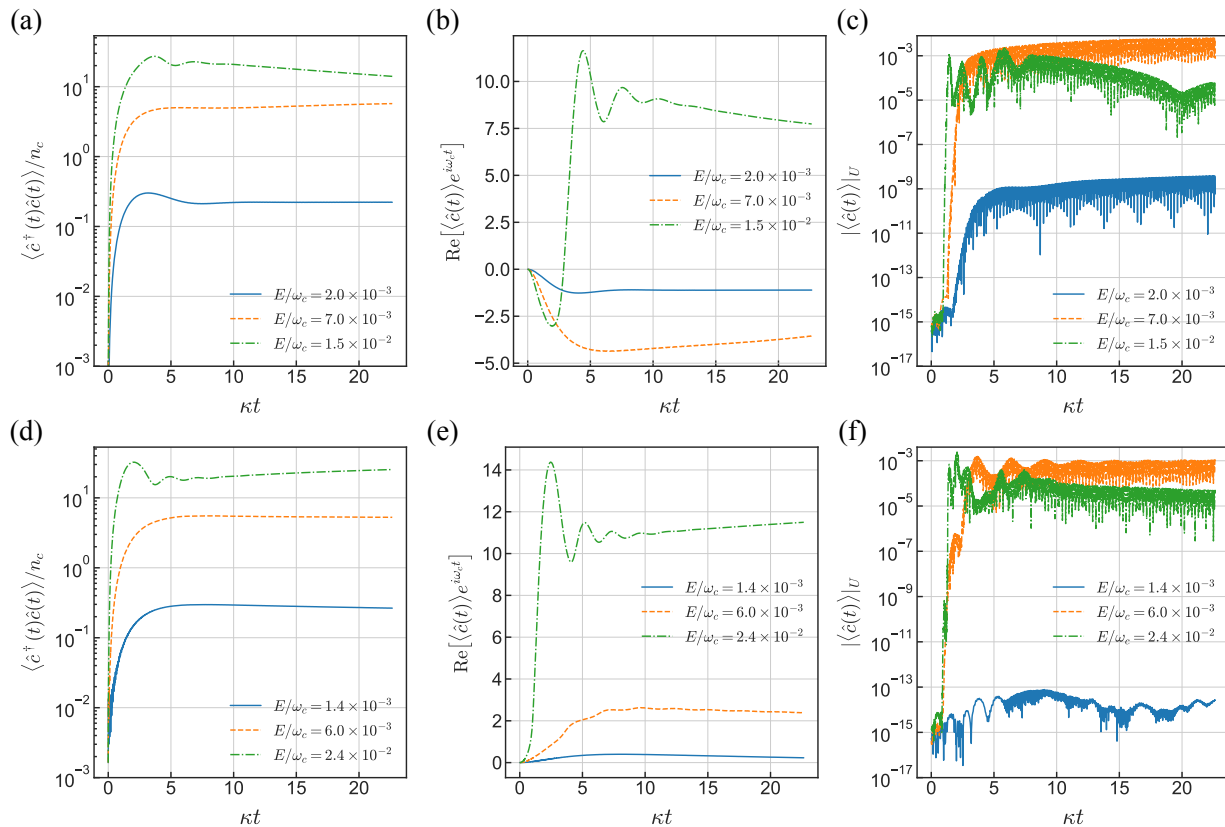
FIG. 8. (a),(d) Time evolution of the cavity photon number for different input-field amplitudes in the transmon cases. (b),(e) Time evolution of the real part of the cavity amplitude in the rotating frame at the drive frequency. (c),(f) Time evolution of the absolute amplitude of the coherent state in the transformed frame starting. Initial states are (a-c) |\tilde{g}, \tilde{0}\rangle and (d-f) |\tilde{e}, \tilde{0}\rangle . The parameters of the system are the same with those in Fig. 7. The highest occupation number N_{\max} is set to 20 in the cases with E/\omega_c = 1.4 \times 10^{-2} and 2.0 \times 10^{-2} , 30 in the case with E/\omega_c = 6.0 \times 10^{-3} , 60 in the case with E/\omega_c = 7.0 \times 10^{-3} , and 100 in the cases with E/\omega_c = 1.5 \times 10^{-2} and 2.4 \times 10^{-2} .
