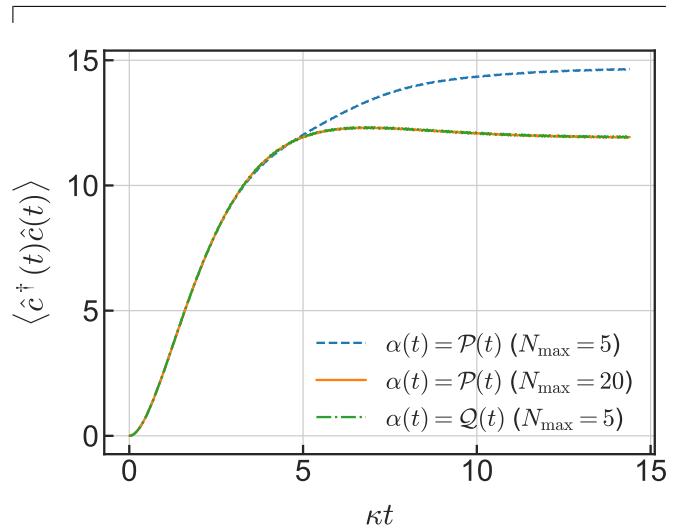
FIG. 2. Time evolution of the cavity photon number under a monochromatic drive Ee^{-i\omega_c t} . The displacement \mathcal{P}(t) is determined by the condition (18), and \mathcal{Q}(t) is determined by our proposed condition (27). N_{\max} is the maximum occupation number of the cavity we set in the simulations. Initially, |\psi_{\text{ini}}\rangle_{qc} is set to |\tilde{g}, \tilde{0}\rangle . The parameters used in the simulation are (\omega_q/\omega_c, g/\omega_c, \kappa/\omega_c, E/\omega_c) = (0.75, 3.0 \times 10^{-2}, 7.2 \times 10^{-3}, 1.0 \times 10^{-2}) .
