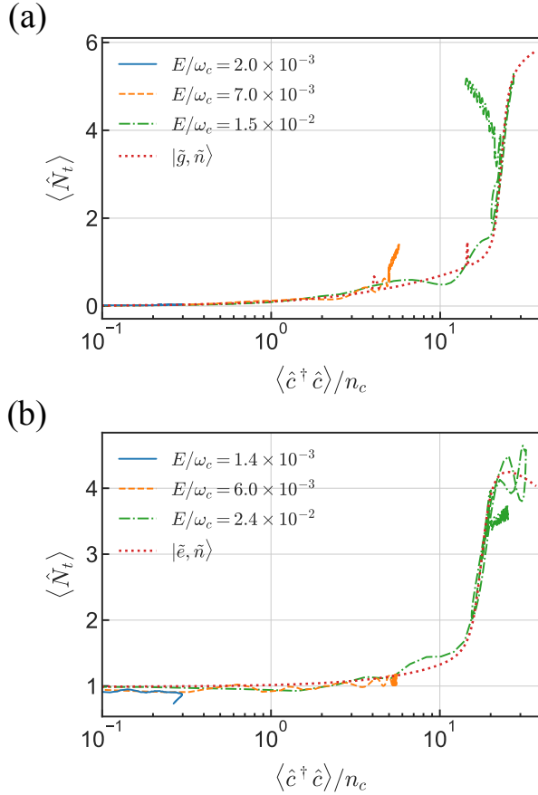
FIG. 9. Parametric plot of the transmon occupation number versus the cavity photon number during the dynamics shown in Fig. 8. Initial states are (a) |\tilde{g}, \tilde{0}\rangle and (b) |\tilde{e}, \tilde{0}\rangle . Red dotted lines represent the transmon occupation numbers as a function of the cavity photon number obtained from the labeled eigenstates |\tilde{g}, \tilde{n}\rangle and |\tilde{e}, \tilde{n}\rangle .
