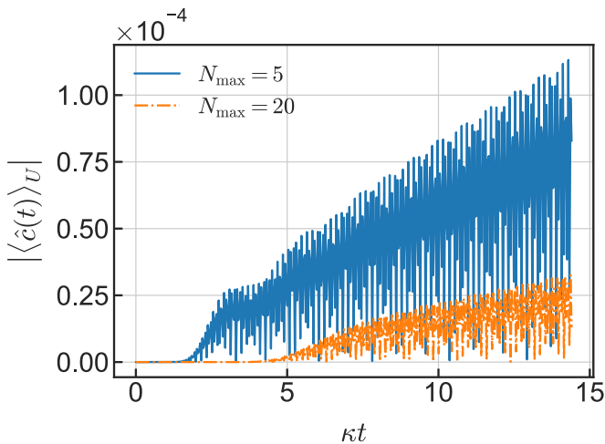
FIG. 3. Time evolution of the absolute amplitude of the coherent state generated in the cavity in the transformed frame. The displacement \alpha(t) is set to \mathcal{Q}(t) . The parameters and the initial state are the same with those in Fig. 2.
