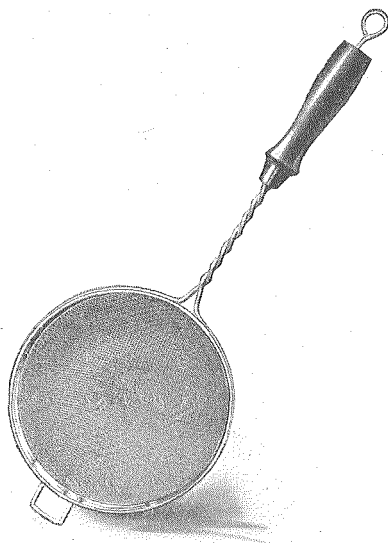
FIG. 58.—Dipper sieve for sifting plaster. It is used by holding it over the plaster bowl, and tapping the rim with the spatula, which assures the plaster reaching the water in a finely divided condition, free from lumps and débris.
